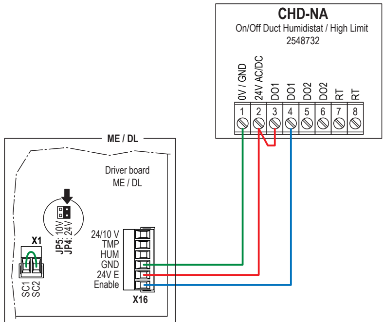
Wiring diagram CHD-NA for DL and ME
