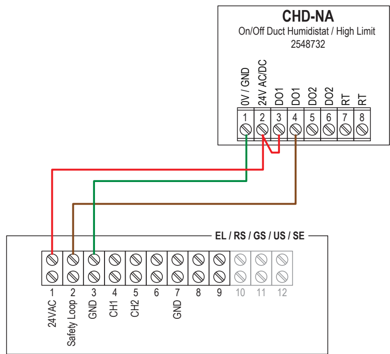
Wiring diagram CHD-NA for RS, EL, GS, US and SE
