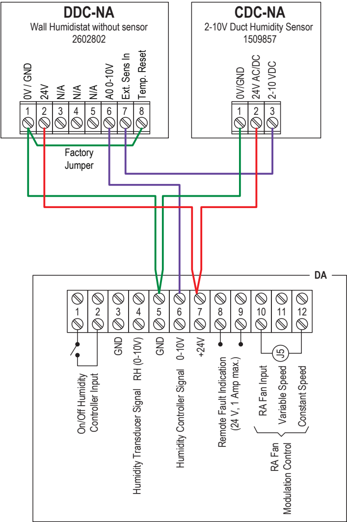
Wiring diagram DDC-NA with CDC-NA for DA
