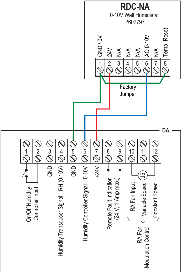
Wiring diagram RDC-NA for DA
